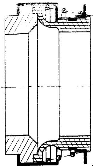
F (Echelle 2:1)
