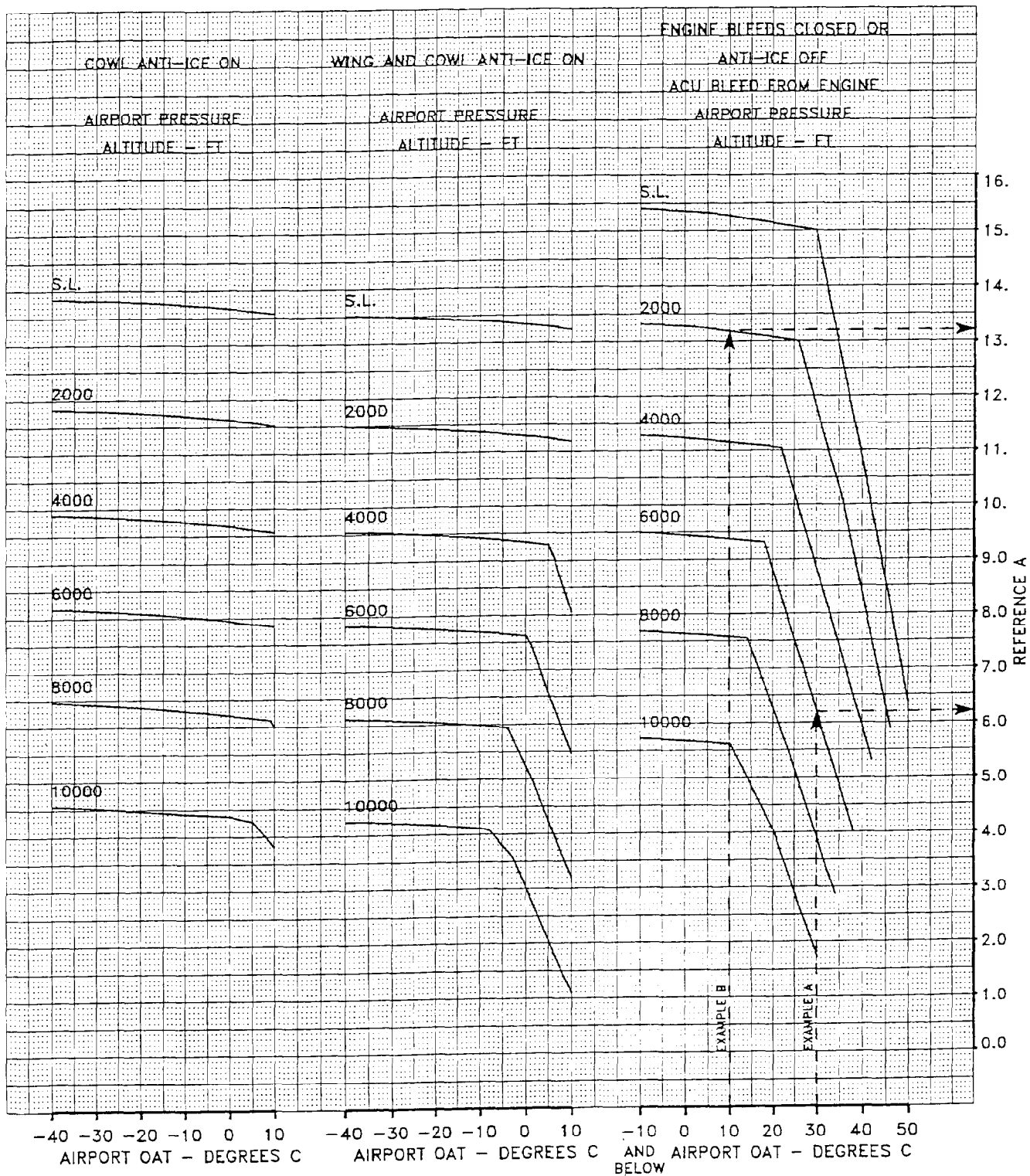
Take-Off Speeds - FLAPS 8 (page 1 of 2) Figure 06-03-14
