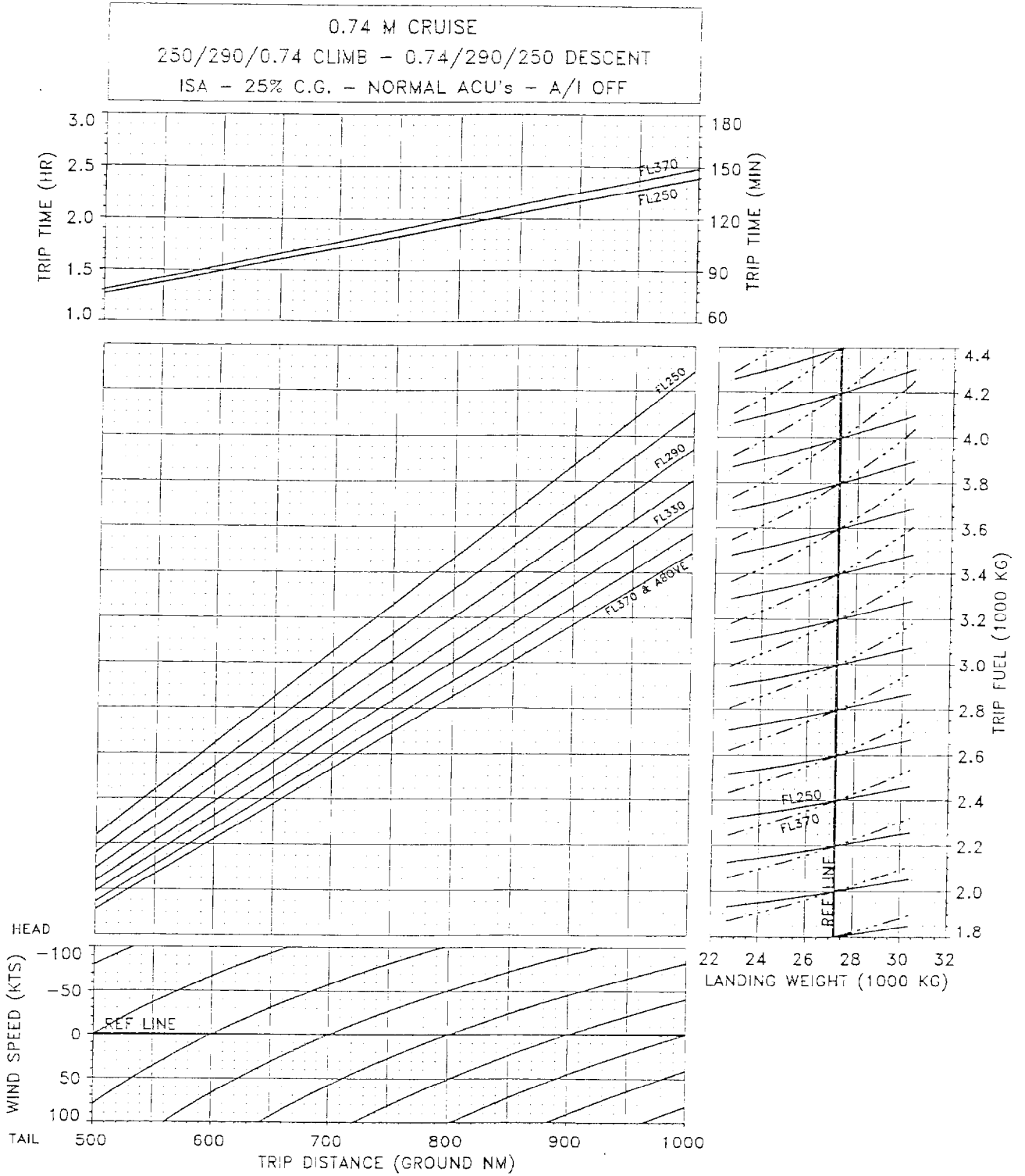
Simplified Flight Planning - 0.74 M (Page 2 of 3) Figure 03-12-1
