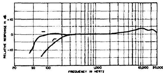
*Curves shown at 1.8m (6 ft) TYPICAL ON-AXIS FREQUENCY RESPONSE FIGURE 1
