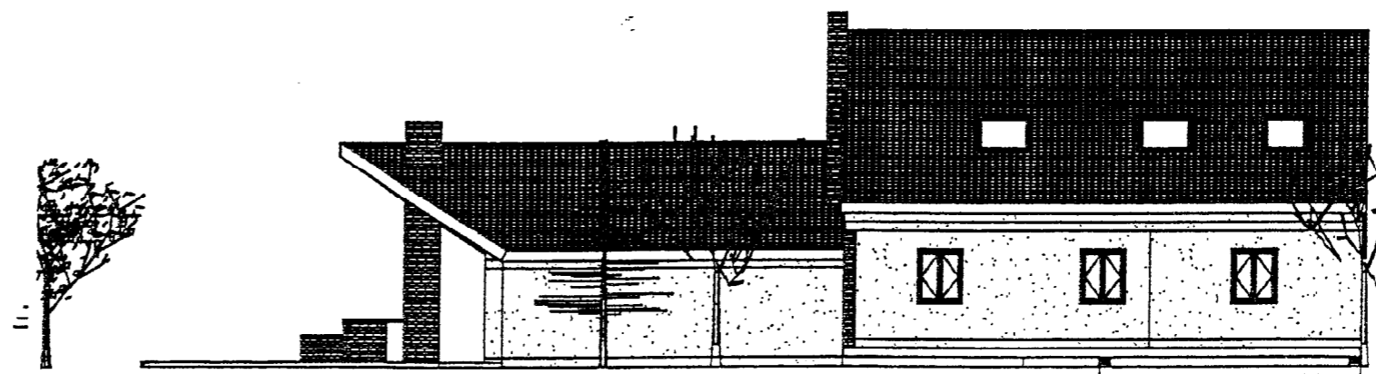
FACADE ARRIERE
