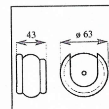
Support entre-murs
