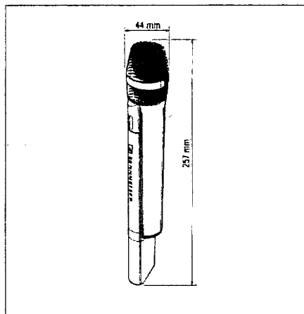
Dimensions SKM 5000
