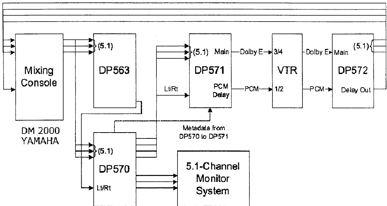
Typical Postproduction Dolby E System
