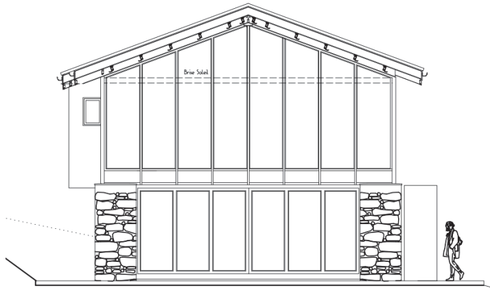
FACADE SUD
