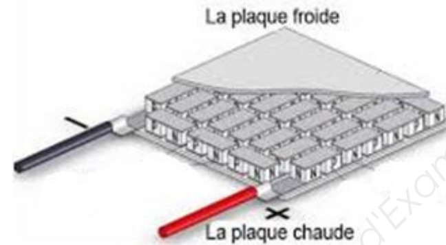
Figure 12 Composant Peltier
