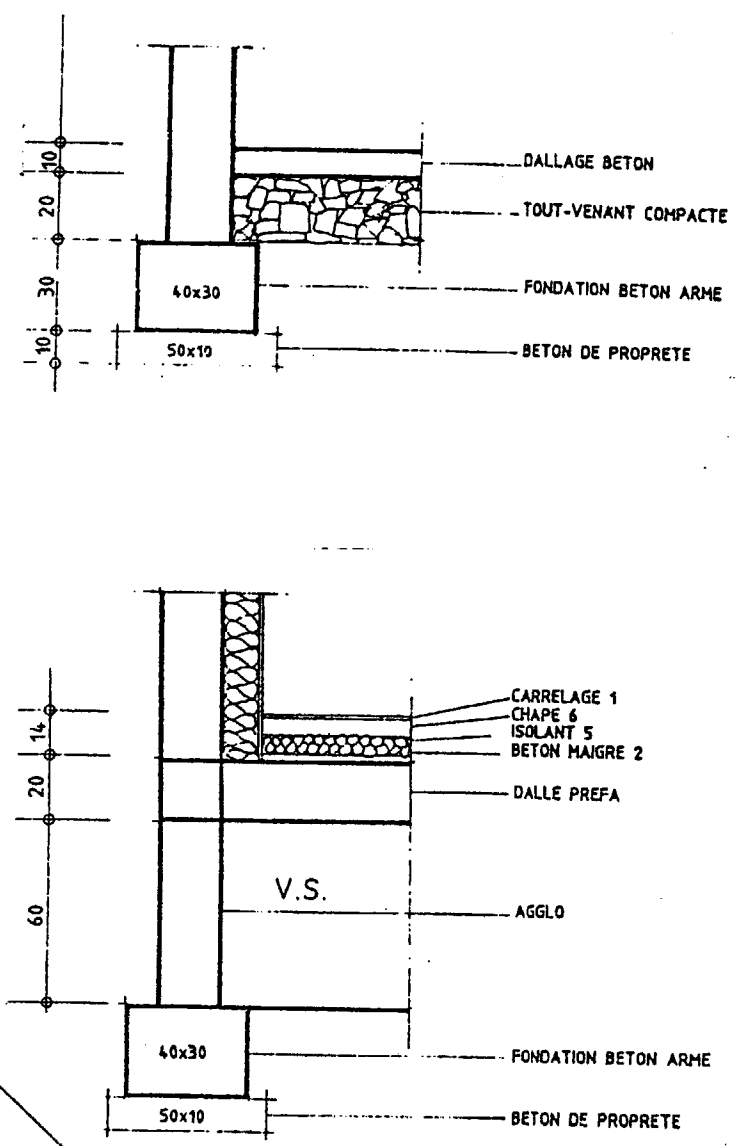
DETAILS FONDATIONS Ech. 1/20 eme
